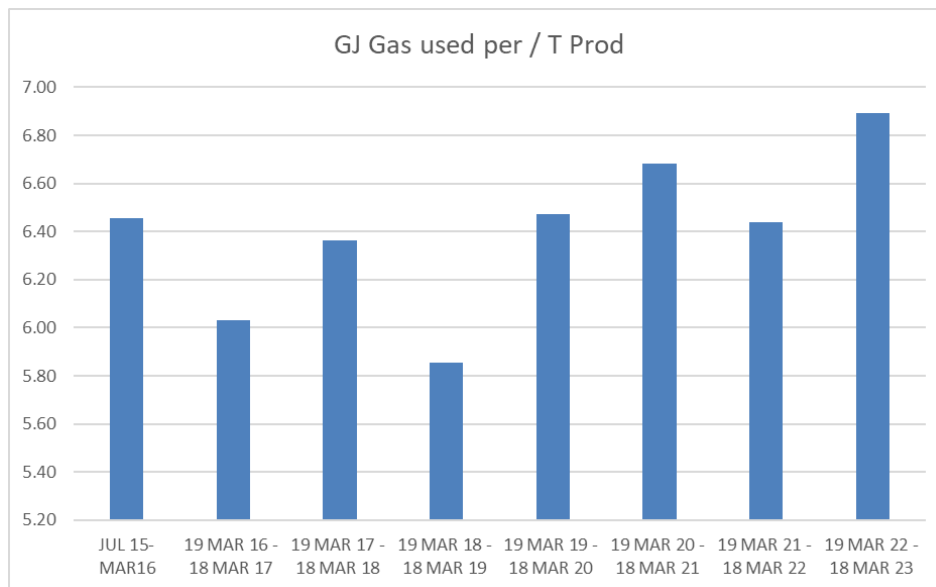
Figure 3: Gas Usage per T Produced
