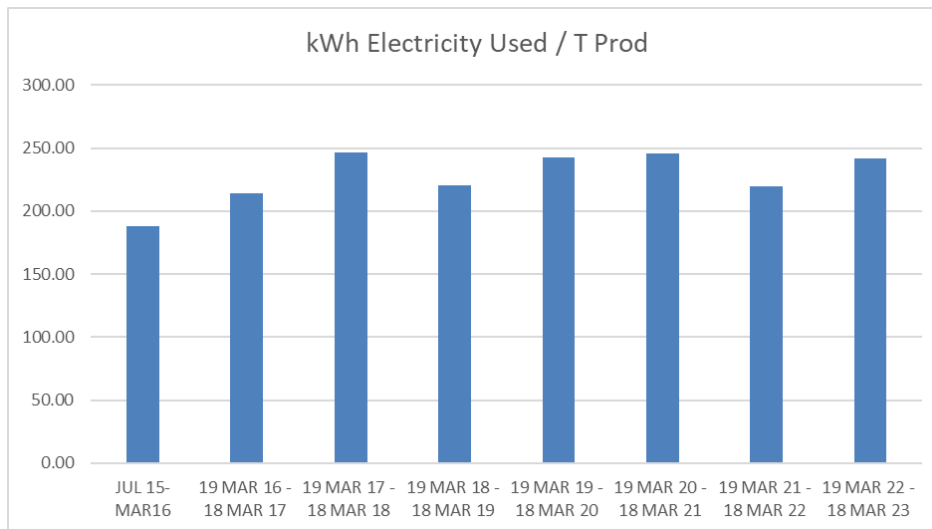
Figure 5: Electricity Used per T Produced
